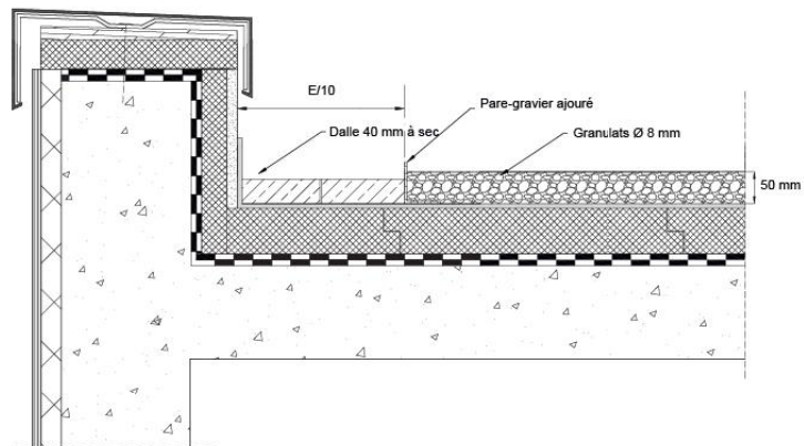
Figure C.3b - Protection P3B
