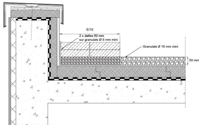
Figure C.6a - Protection P6A
