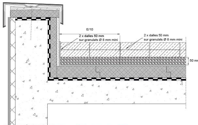
Figure C.6b - Protection P6B
