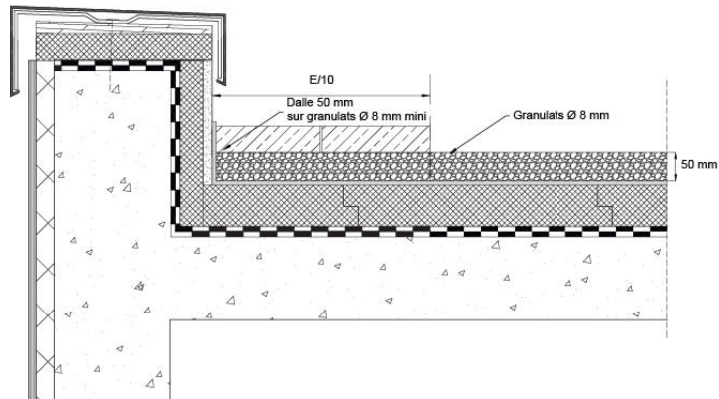
Figure C.3a - Protection P3A
