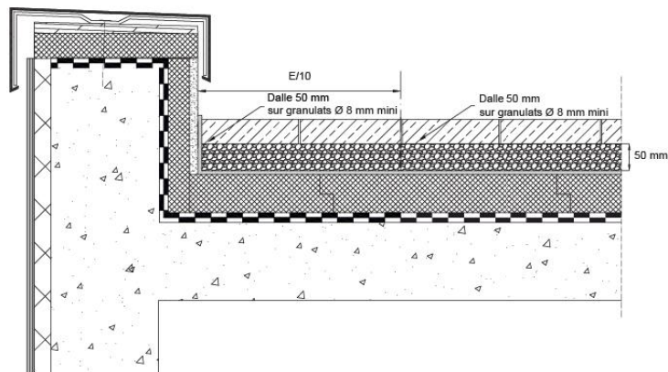
Figure C.3c - Protection P3C
